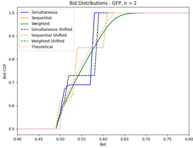
Figure 1: Bidder dynamics run for 100 and 101 trials for GFP, n = 2 , \pi = \frac{1}{2} .
