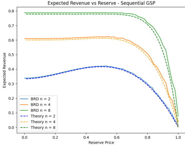
Figure 12: Shown above is the reserve vs. expected revenue for each of n = 2, 4, 8 using sequential learning in GSP. Like above, we have shown the bidder behavior converges to the theoretical in the sequential setting.
