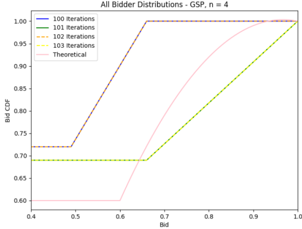
Figure 14: We run BRD on GSP for 100, 101, 102, and 103 iterations at \pi = \frac{1}{2} , n = 4 respectively to see that the bidder behavior cycles in periods of 2. Again, the theoretical equilibrium here is seemingly off due to the \alpha_1 scaling issue.
