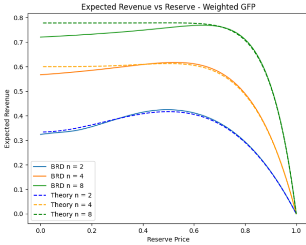
Figure 10: Shown above is the reserve vs. expected revenue for each of n = 2, 4, 8 using weighted learning in GFP.
