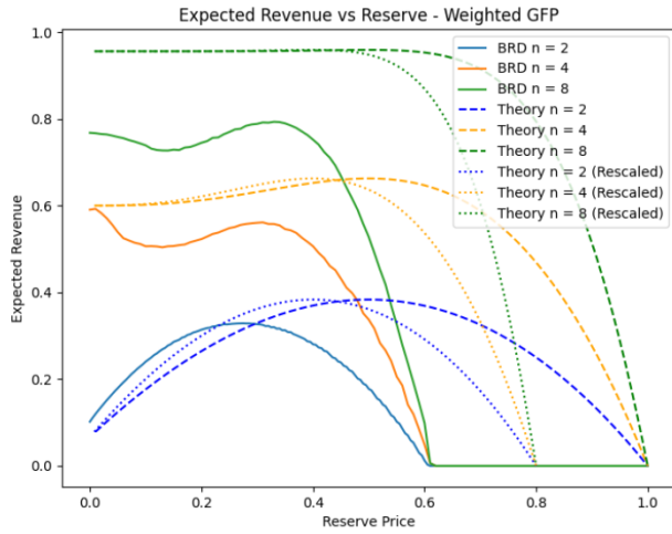
Figure 18: GFP, weighted learning. Unlike the revenue curves above, the revenue curves terminate at 0.6, though the shapes of the curves vaguely resembles that of the theoretical. Interestingly, this is because the bidder distributions recovered by GFP terminate at 0.6; and as the bidding distributions recovered quickly converge this pseudo-equilibrium, then there is no incentive to ever bid larger than 0.6
