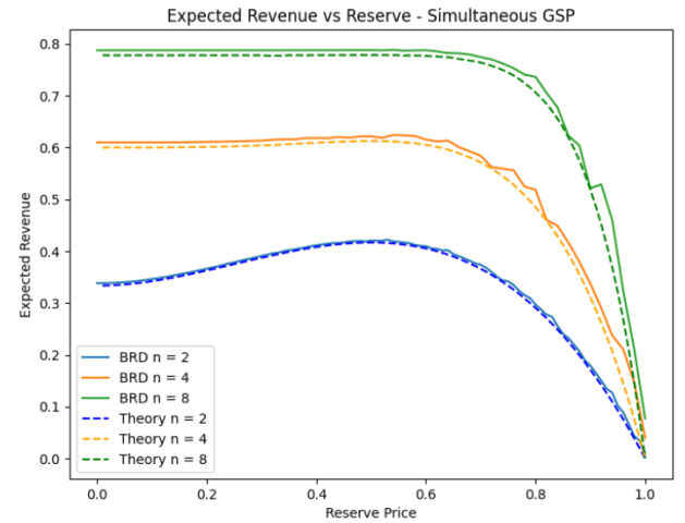
Figure 11: Shown above is the reserve vs. expected revenue for each of n = 2, 4, 8 using simultaneous learning in GSP.
