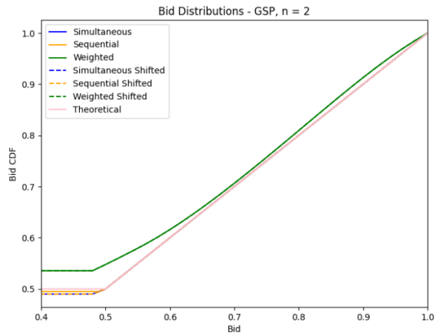
Figure 4: Bidder dynamics run for 100 and 101 trials for GSP, n = 2 .
