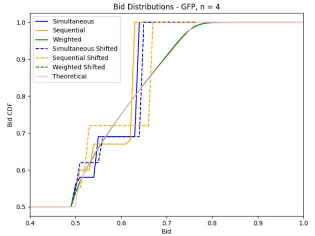
Figure 2: Bidder dynamics run for 100 and 101 trials for GFP, n = 4 , \pi = \frac{1}{2} .
