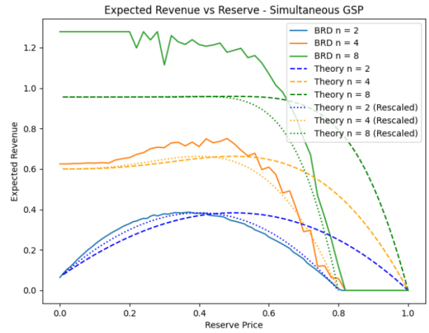
Figure 19: GSP, simultaneous learning. Here, like in the GFP simultaneous, we have cycling behavior which yields noisy revenue curves and a similar horizontal scaling factor of 0.8. The curves are noticeably less noisy than that of the GFP, though, and but also overshoot (rather than undershoot) the theoretical equilibrium revenues.
