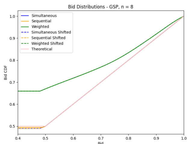
Figure 6: Bidder dynamics run for 100 and 101 trials for GSP, n = 8 .
