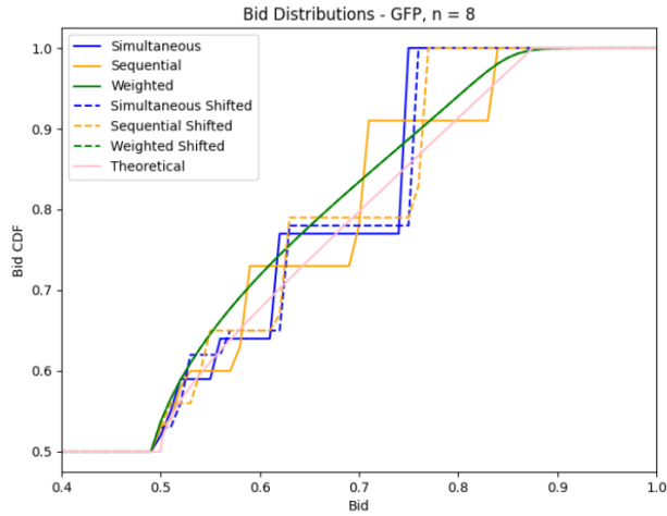
Figure 3: Bidder dynamics run for 100 and 101 trials for GFP, n = 8 , \pi = \frac{1}{2} .
