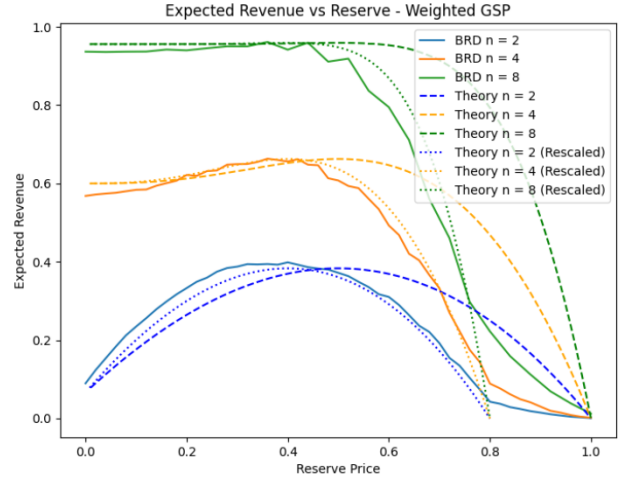
Figure 21: GSP, weighted learning. Even more so than the sequential learning version, weighted learning almost recovers the theoretical revenue curves (up to a scaling constant of 0.8). Furthermore, it immediately recovers a symmetric bidding distribution, though due to the exponentially weighted scheme, puts some non-negative mass in the bidder distributions above 0.8 which results in having positive revenue past a reserve of 0.8.
