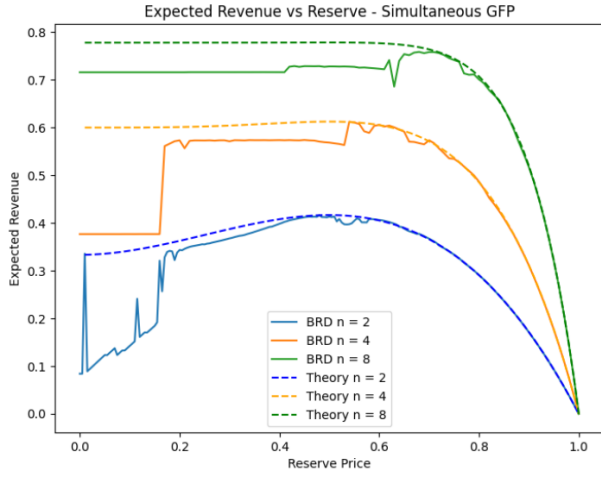
Figure 8: Shown above is the reserve vs. expected revenue for each of n = 2, 4, 8 using simultaneous learning in GFP.
