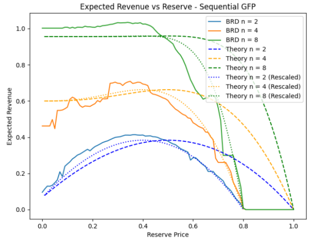
Figure 17: GFP, sequential learning. Like above, the cycling in GFP yields noisy expected revenue curves; though the effect is less apparent than in simultaneous learning. Once again, we see that the recovered revenue curves are a horizontally scaled version (also by 0.8) version of the theoretical revenue curves.
