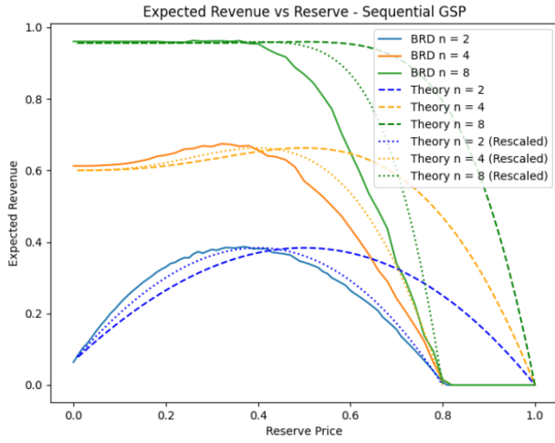
Figure 20: GSP, sequential learning. This is the more well recovered revenue curves (up to the scaling constant of 0.8) as despite the bidder behavior cycling and not converging to a symmetric equilibrium, the bidder's behave very similarly suggesting that a symmetric equilibrium is nearby.
