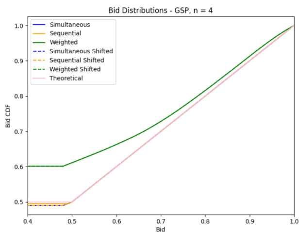
Figure 5: Bidder dynamics run for 100 and 101 trials for GSP, n = 4 , \pi = \frac{1}{2} .
