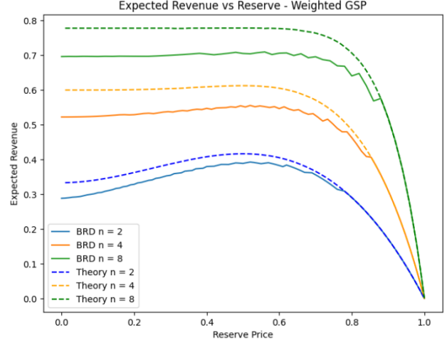
Figure 13: Shown above is the reserve vs. expected revenue for each of n = 2, 4, 8 using weighted learning in GSP.
