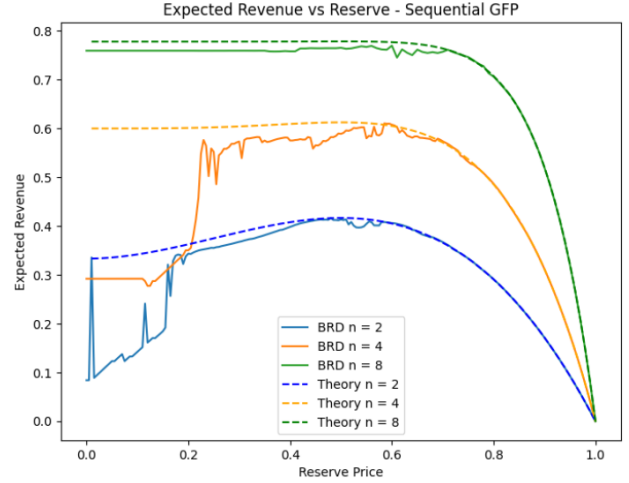
Figure 9: Shown above is the reserve vs. expected revenue for each of n = 2, 4, 8 using sequential learning in GFP.
