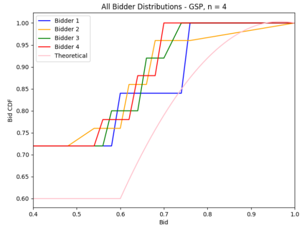
Figure 15: We run SBRD on GSP for 100 iterations at \pi = \frac{1}{2} , n = 4 and the bidder distributions do not converge, nor are they symmetric. Note that the bids are generally smaller than the theoretical.
