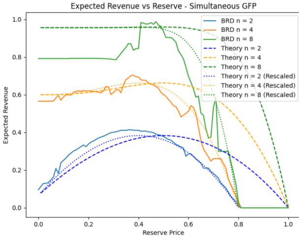
Figure 16: GFP, simultaneous learning. We note that we once again observe noise due the cycling behavior as we saw in the GFP, one item, and simultaneous learning setting. The obtained curves is a horizontally-scaled (by roughly 0.8) version of the theoretical revenue, which is due to the assumption that \alpha_1 = 1 in the papers in which they were derived. It is also apparent that the cycling behavior actually worsens as the number of bidders increases.
